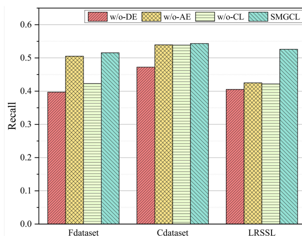
Figure 2. The Recalls of all compared approaches obtained in 10-CV.
